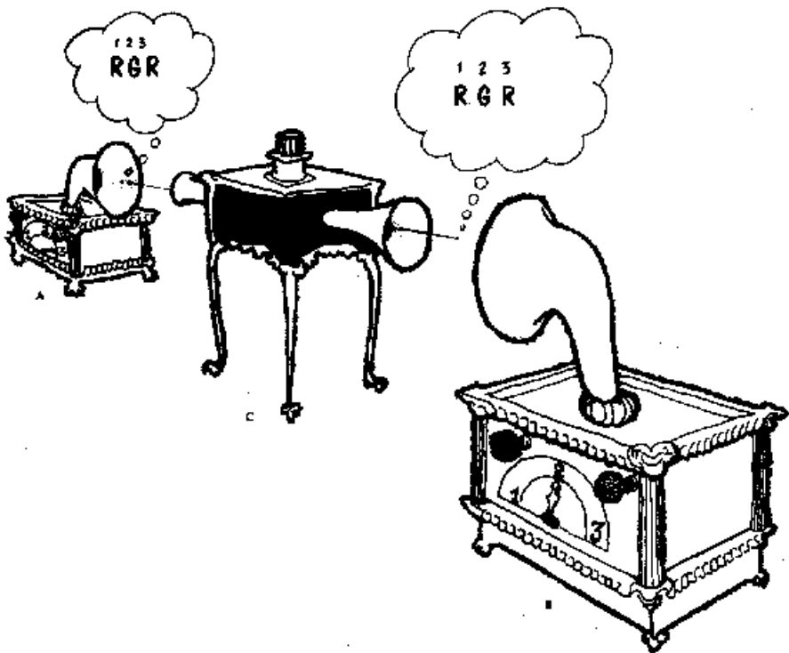
Figure 7 – Instruction sets.
